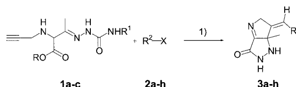
Scheme 1. Reagents and conditions: 1) Pd(OAc) 2 , DPPF, piperidine, RT, 24 h. Spectroscopic data of new compounds can be found in the Supporting Information.
